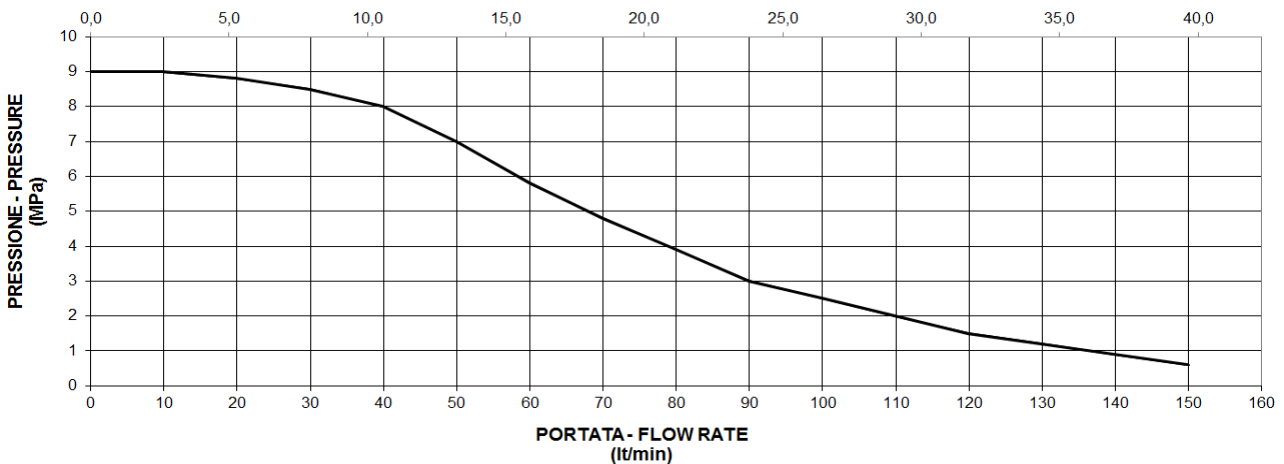
DIAGRAMMA PORTATA - PRESSIONE PRESSURE-FLOW RATE DIAGRAM
